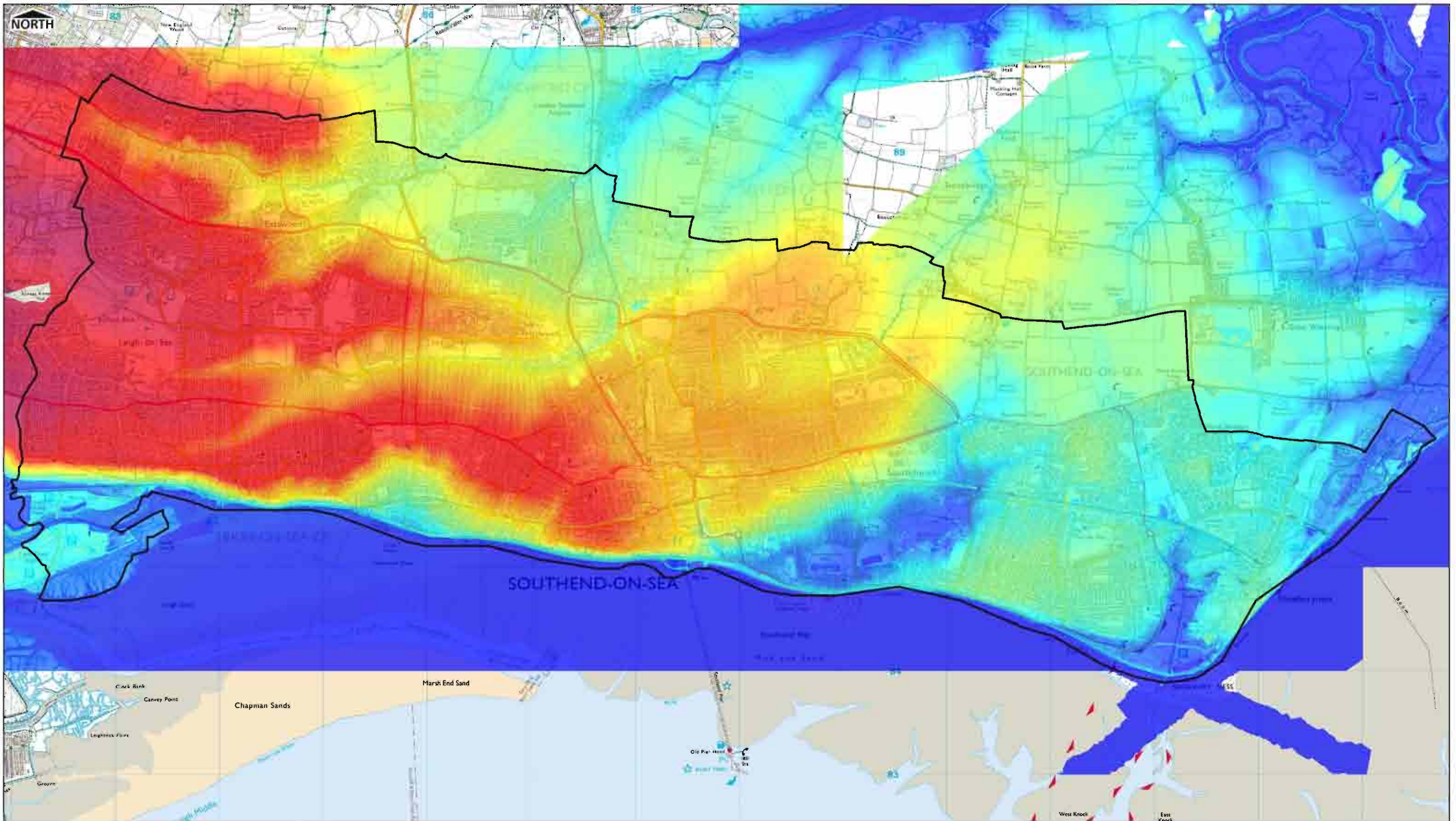
FIGURE 3 - TOPOGRAPHY (LIDAR)
